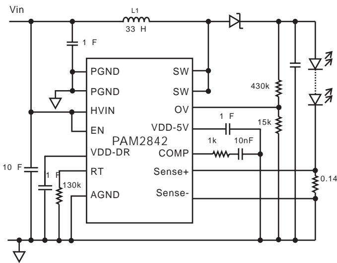
Boost with Low Side Current Sense
